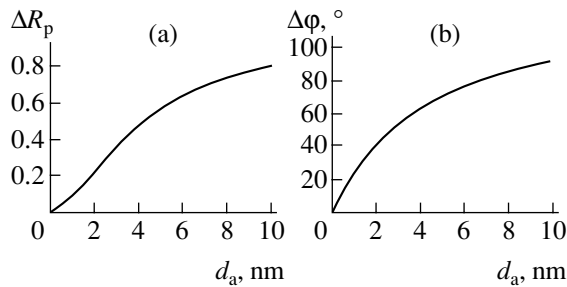
Fig. 2. Calculated curves of the (a) \Delta R_p and (b) \Delta\phi versus thickness d_a of a LiF layer on a 45.5-nm-thick copper film, in which SEWs are excited by the radiation with \lambda = 632.8 nm via an ATR prism with n_p = 1.51 .
